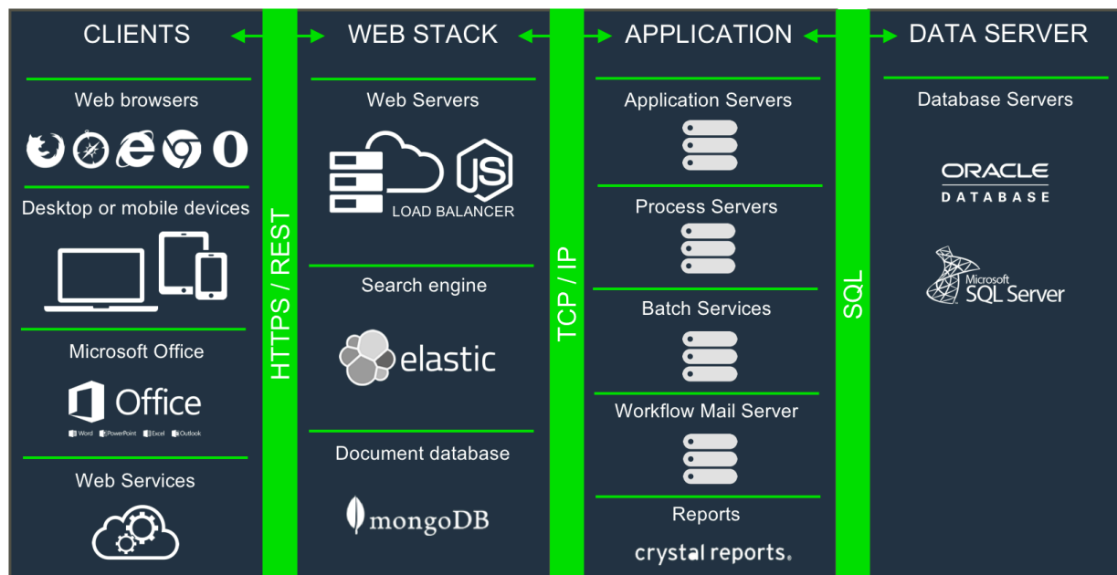
Sage X3 system architecture
